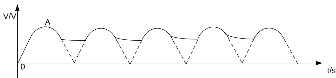
Smoothed output of a full – wave rectifier
